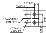
PRIMARY BUSHING DETAIL
