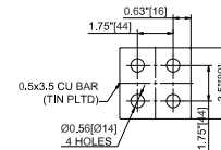
SECONDARY BUSHING DETAIL
