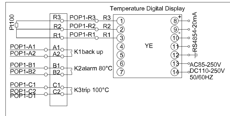
OIL TEMPERATURE INDICATORS
